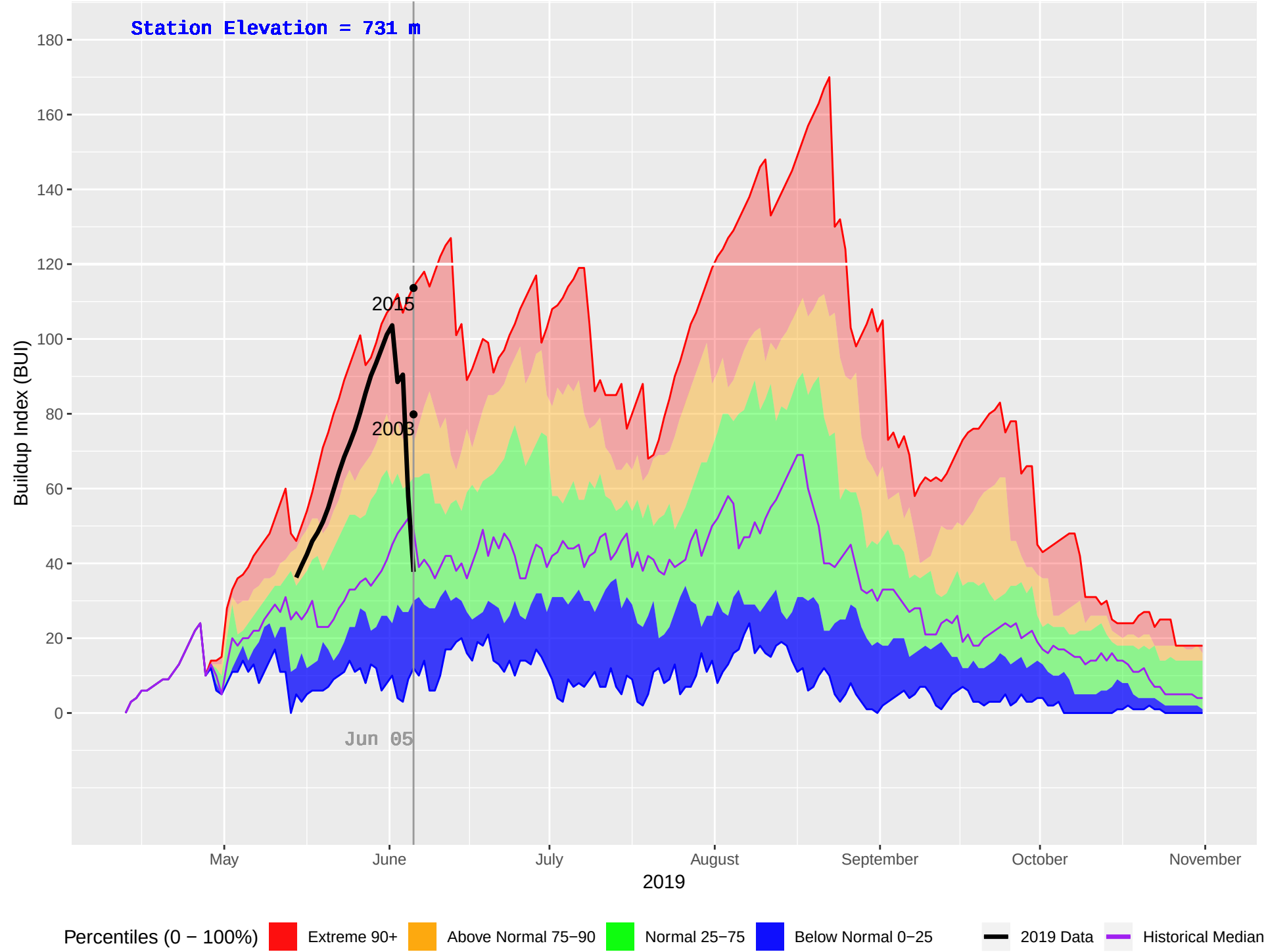
FIRESIDE (440) : Historical (1996–2018), Current (2019) Daily Buildup Index (BUI)
