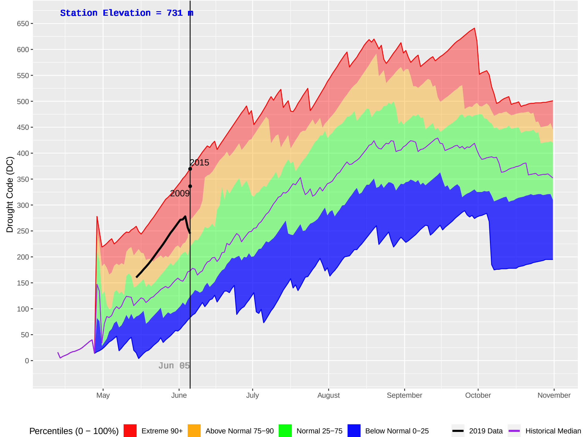
FIRESIDE (440) : Historical (1996–2018) and Current (2019) Daily Drought Code (DC)
