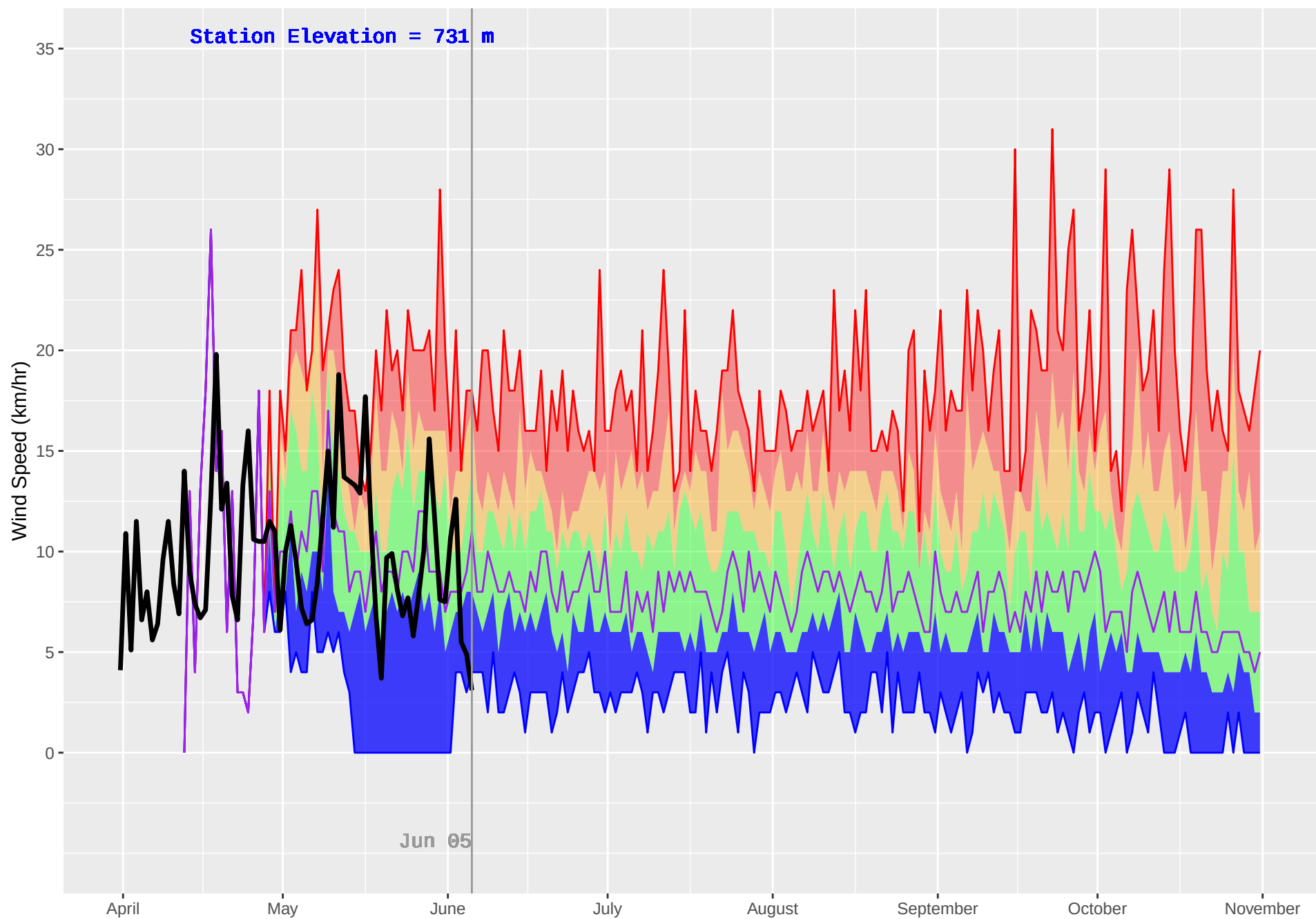
FIRESIDE (440) : Historical (1996–2018) and Current (2019) Daily Wind Speed
