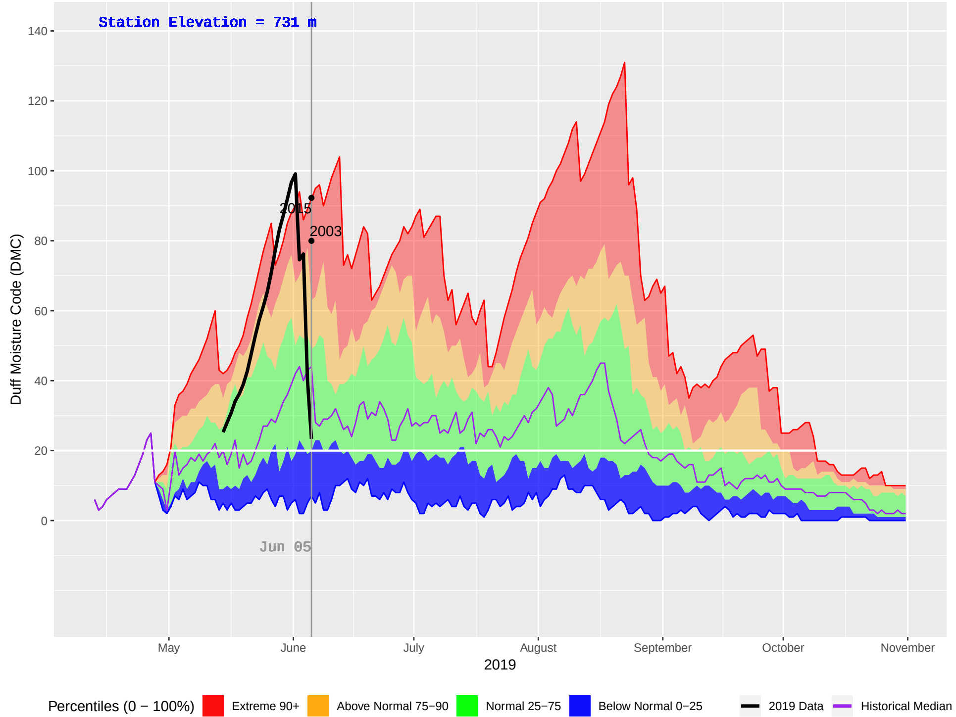
FIRESIDE (440) : Historical (1996–2018), Current (2019) Daily Duff Moisture Code (DMC)
