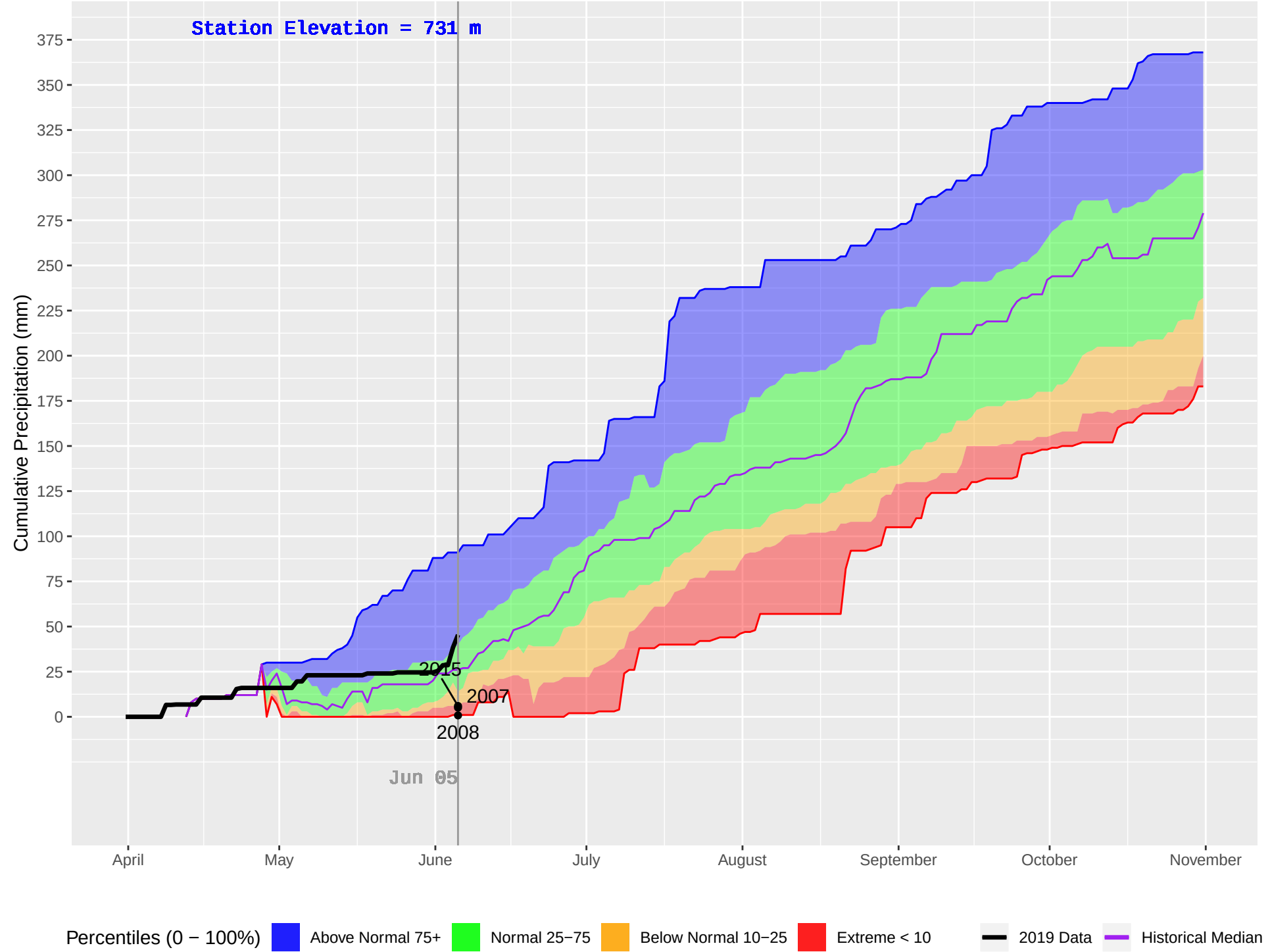
FIRESIDE (440) : Historical (1996–2018), Current (2019) Daily Cumulative Precipitation
