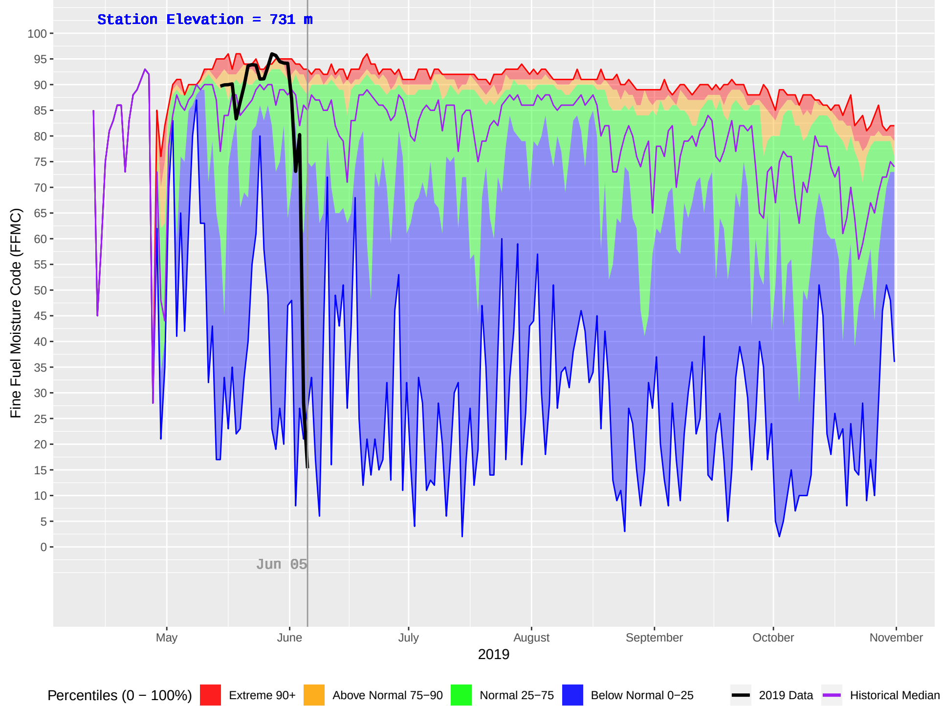
FIRESIDE (440) : Historical (1996–2018) and Current (2019) Daily Fine Fuel Moisture Code (FFMC)
