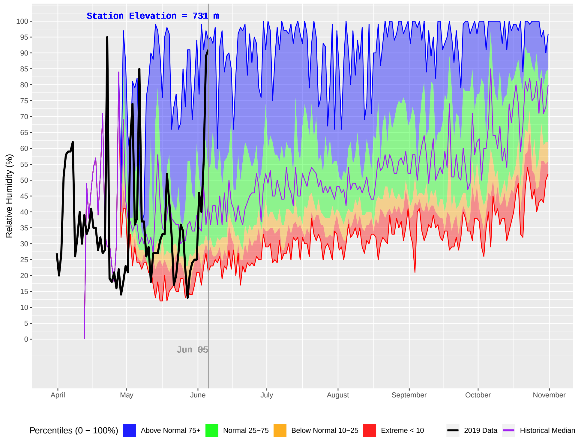
FIRESIDE (440) : Historical (1996–2018) and Current (2019) Daily Relative Humidity
